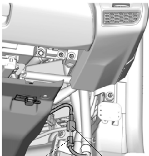
VEHICLE 2-PIN CONNECTOR (red and black wires)
