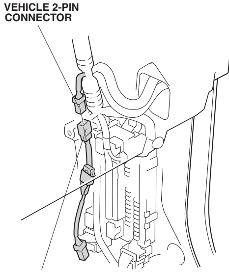
VEHICLE 2-PIN CONNECTOR DOOR SILL TRIM HARNESS 2-PIN CONNECTOR
