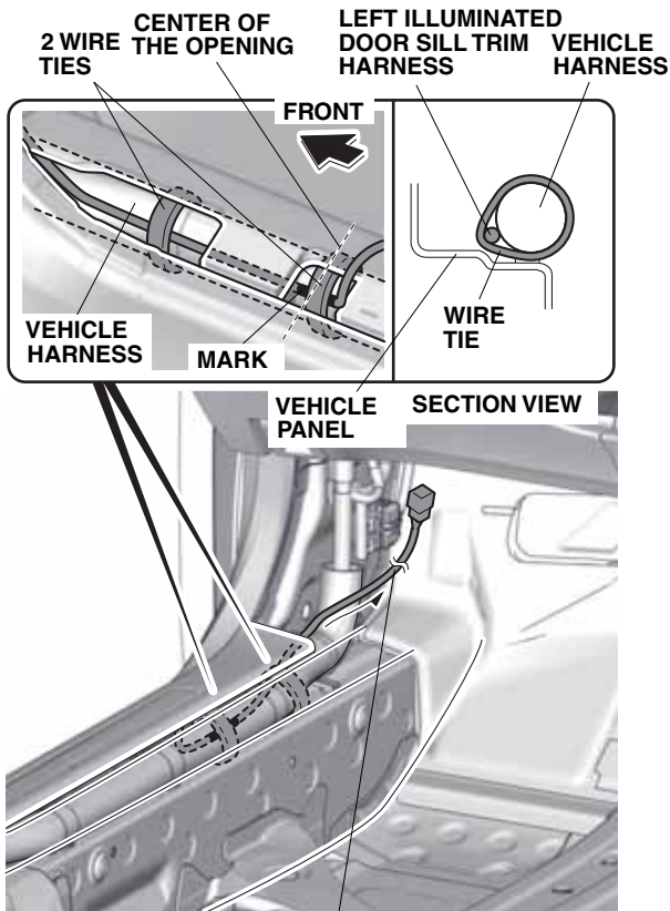
LEFT ILLUMINATED DOOR SILL TRIM HARNESS QCN1108CG
