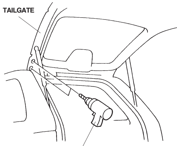
First drill pilot holes with a 3 mm bit, and finish with an 8 mm bit.
